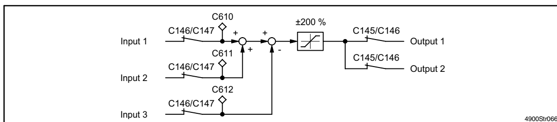
FIG 7-39 Addition 1
