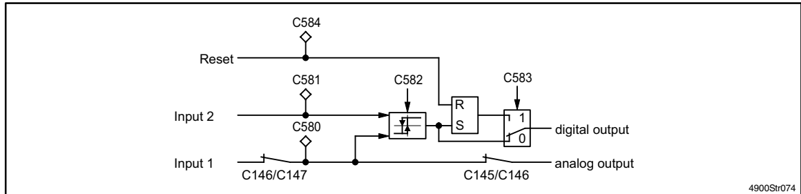
FIG 7-47 Comparator 1
