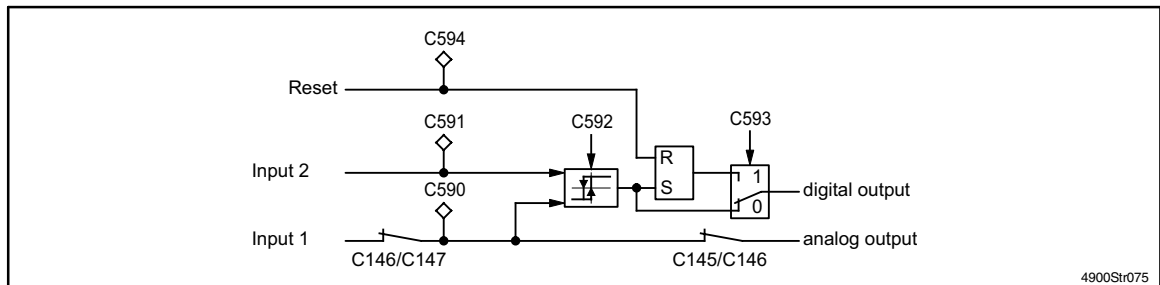
FIG 7-48 Comparator 2
