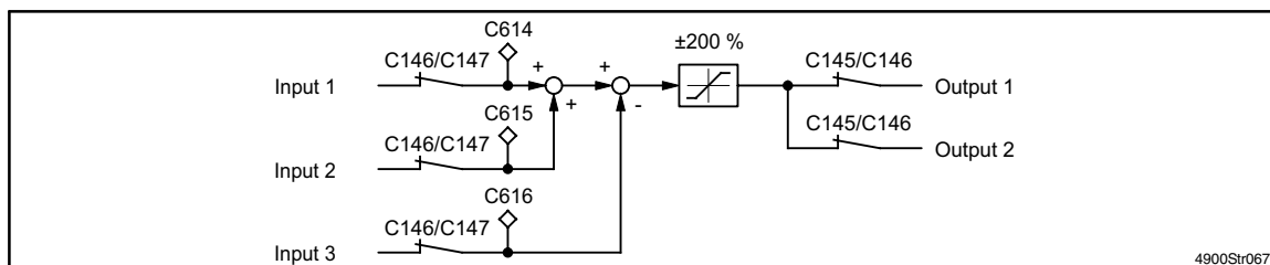
FIG 7-40 Addition 2
