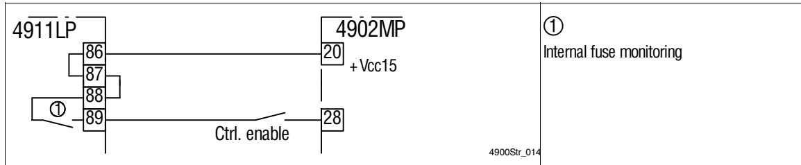
FIG 4-14 4811...4813 and 4911...4913
