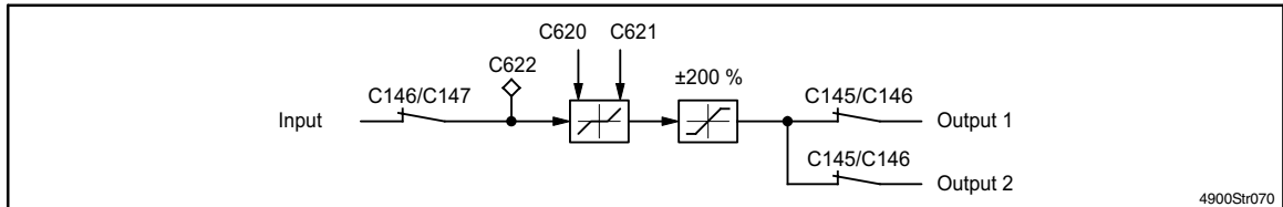
FIG 7-43 Dead-band element
